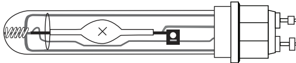
PGZX18 T12 (Clear, Double Envelope)
