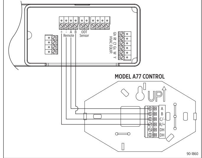
FIGURE 7 – MODEL A77 REMOTE CONTROL WIRING
