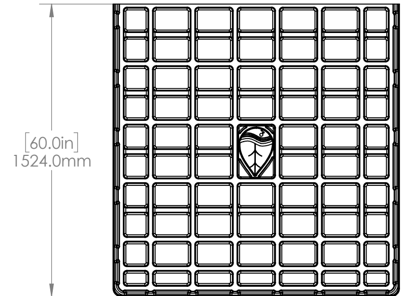
BOTANICARE 5'Wx5'L END TRAY BLACK ABS/1 HGC706668 27.07 lbs
