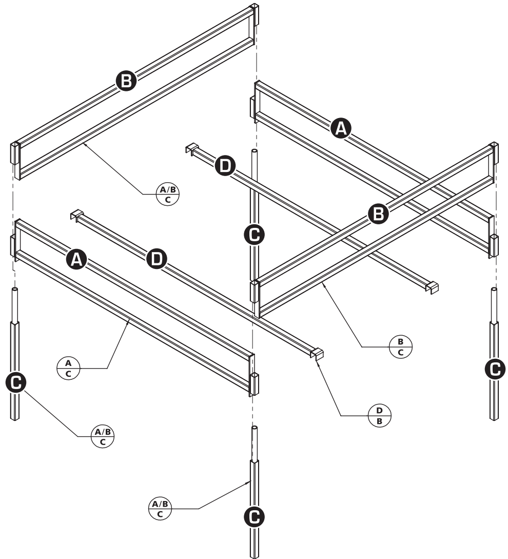
C - LEG STANDS
